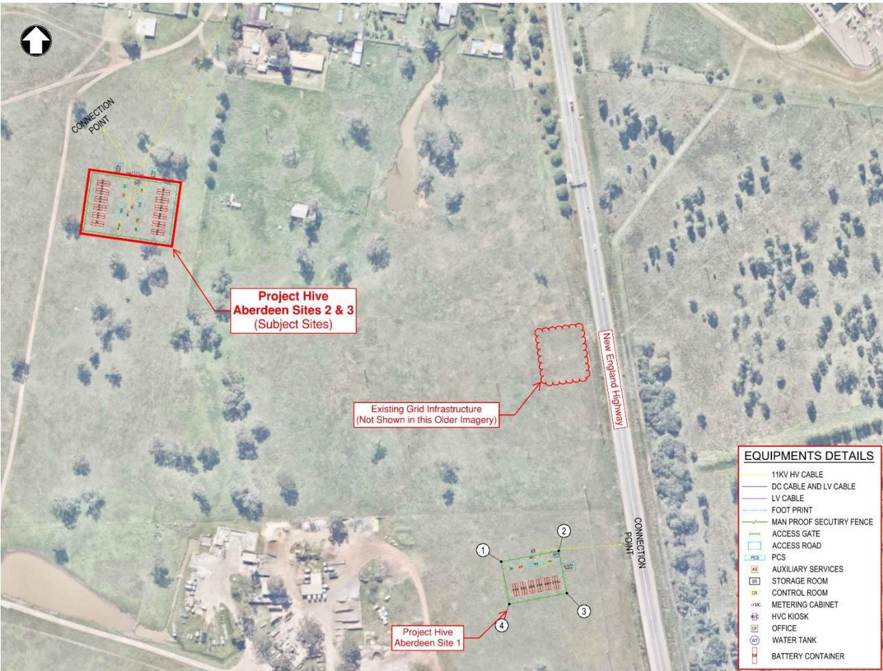
Figure 1: Site Overview and Equipment Layout
